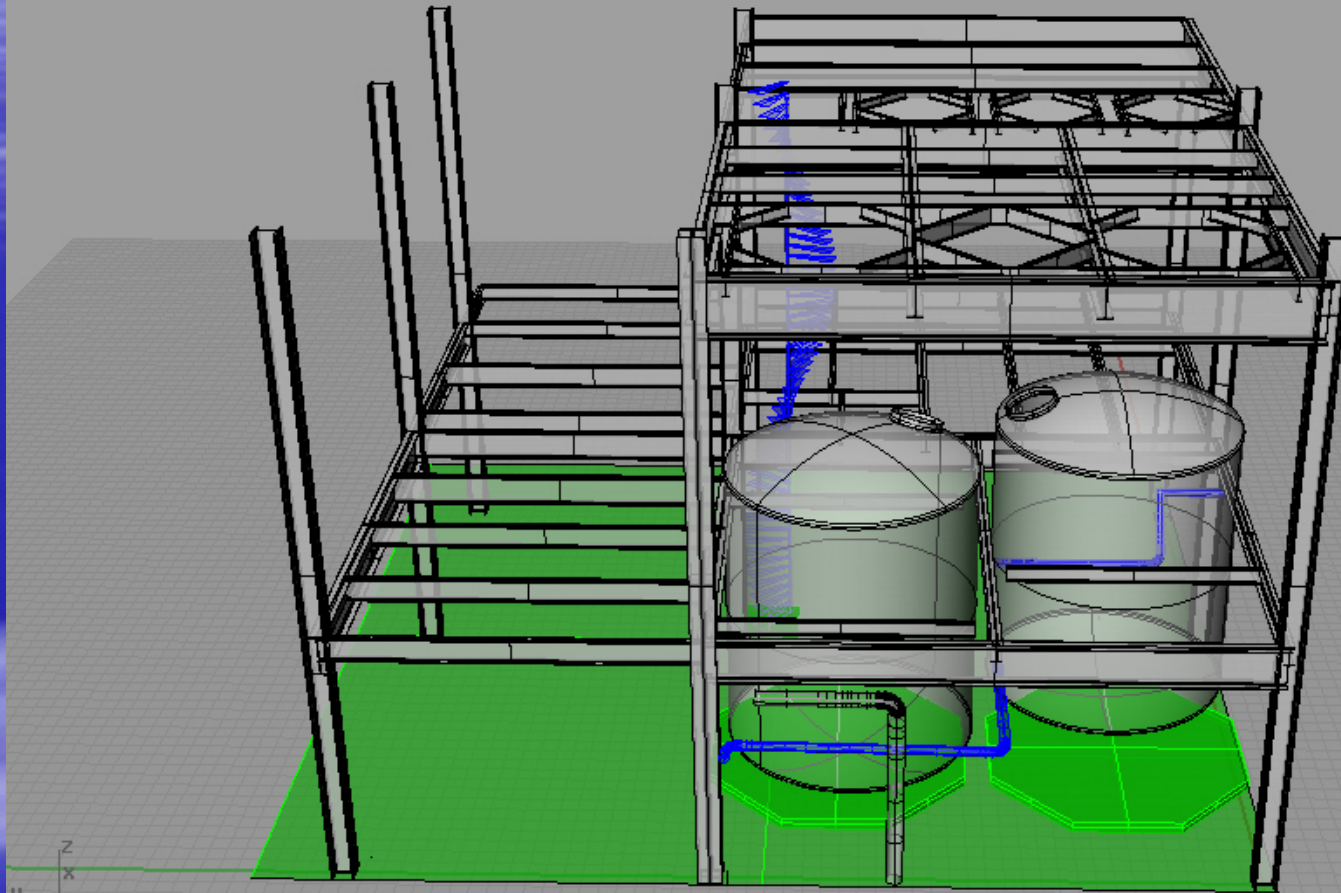
Model of a chemical production facility
